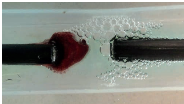
Microelectrolysis of copper chloride solution, close-up
