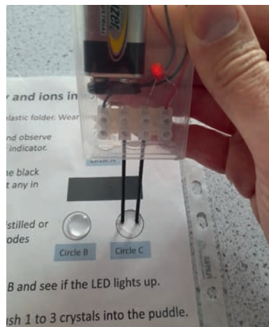
Conductivity meter in a drop of distilled water with crystals of sodium chloride added
