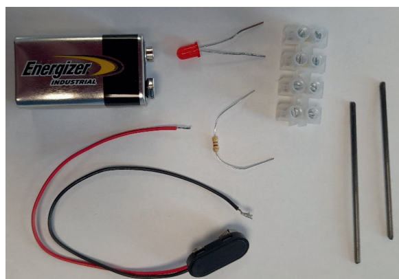
Conductivity meter components
